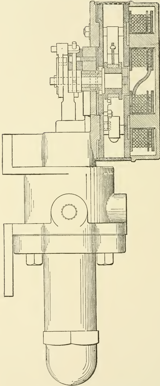
Fig. 91. Part Section of Pump Governor
